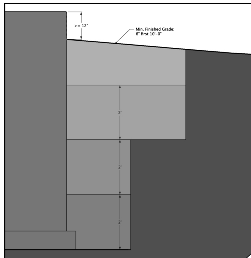
Fig 7: Backfill in tamped lifts and finish with proper slope
