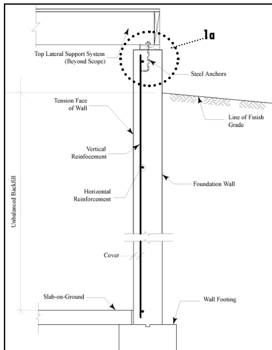
Fig 1: Typical simply-supported foundation wall
