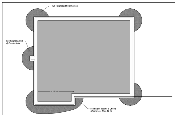
Fig 5: Common allowable areas for full-height backfill
