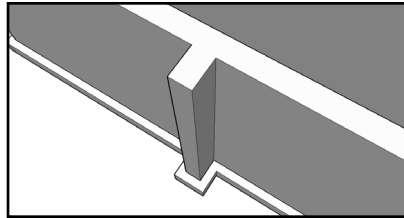
Fig 6: A counterfort monolithic with the foundation wall will support longer wall lengths like an offset or corner
